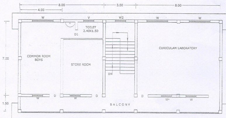
SECOUND FLOOR PLAN
